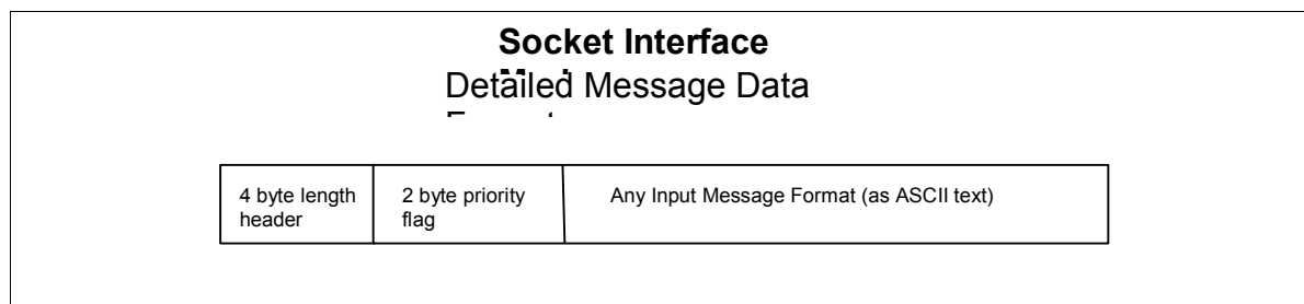
Figure 10. The detailed message data format for the socket interface mode
