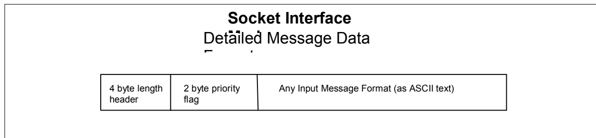
Figure 11. The detailed message data format for the socket interface mode
