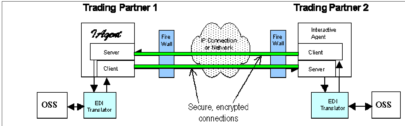
Figure 2. Using an IAgent3 system for IA trading partner communications
